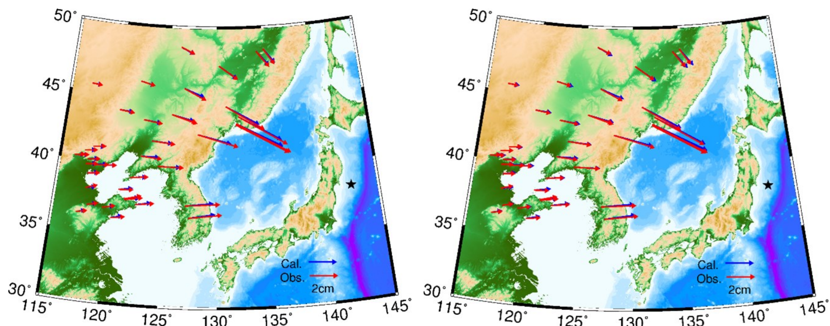
Figure. 1 Far-field horizontal co-seismic displacements of the 2011 Mw 9.0 Tohoku earthquake (left) and with the adjusted fault slip model (right).
