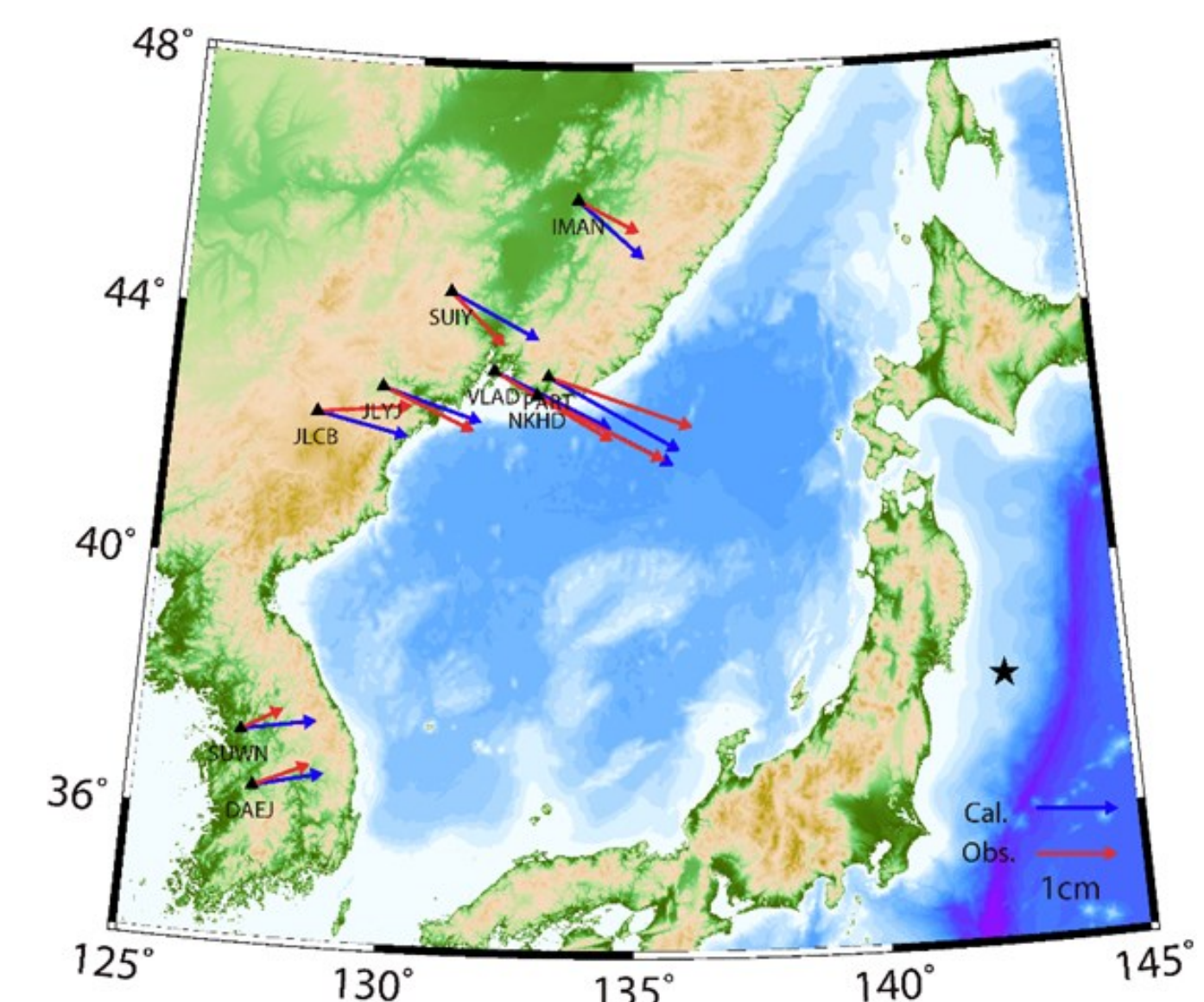
Figure. 2 Comparison between accumulated post-seismic deformations observed from nine far-field GPS stations and modeled from 2.5 to 4.5 years after the Mw9.0 earthquake. The red arrows indicate the GPS results; the blue arrows show the fitted results from the viscoelastic spherical dislocation theory at a viscosity of 1 \times 10^{19} Pa·s
