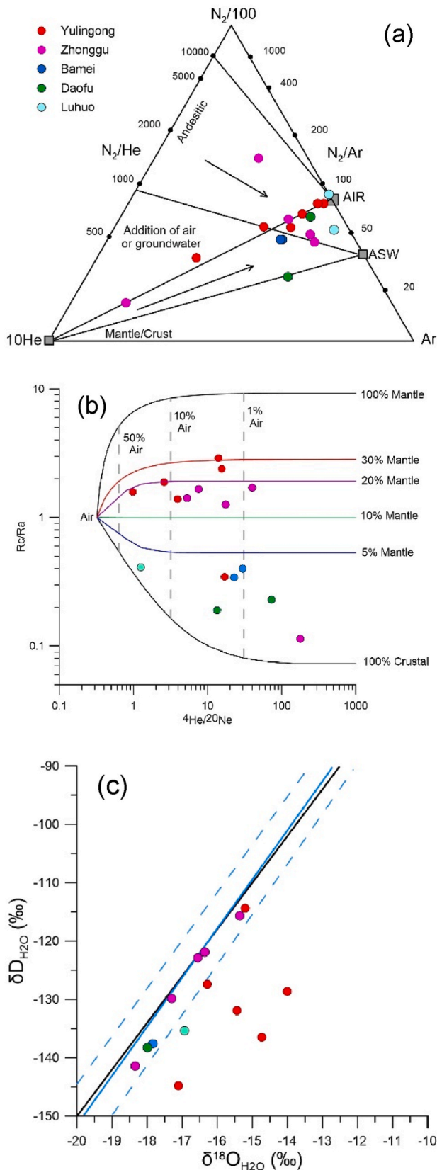
Fig. 3. Plot of (a) N_2 -He-Ar; (b) He/Ne ratios versus the Rc/Ra ratios, where the mixing-boundary lines are built from the method proposed by Sano and Wakita [69]; (c) \delta^2H_{H_2O} versus \delta^{18}O_{H_2O} , the black solid line represents the global meteoric water line (GMWL: \delta^2H = 8\delta^{18}O + 10 ), the blue solid and dashed lines represent the regional meteoric water line with confidence interval for the Tibetan Plateau domain \delta^2H = (8.41 \pm 0.20)\delta^{18}O + (16.72 \pm 2.98) [70].
