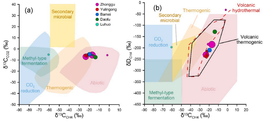
Fig. 7. Methane genetic diagrams based on (a) \delta^{13}\text{C}_{\text{CO}_2} versus \delta^{13}\text{C}_{\text{CH}_4} ; (b) \delta^2\text{D}_{\text{CH}_4} versus \delta^{13}\text{C}_{\text{CH}_4} .
