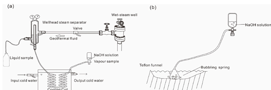
Fig. 2. Sampling methods using the Giggenbach bottle at (a) geothermal wells and (b) bubbling springs, respectively.
