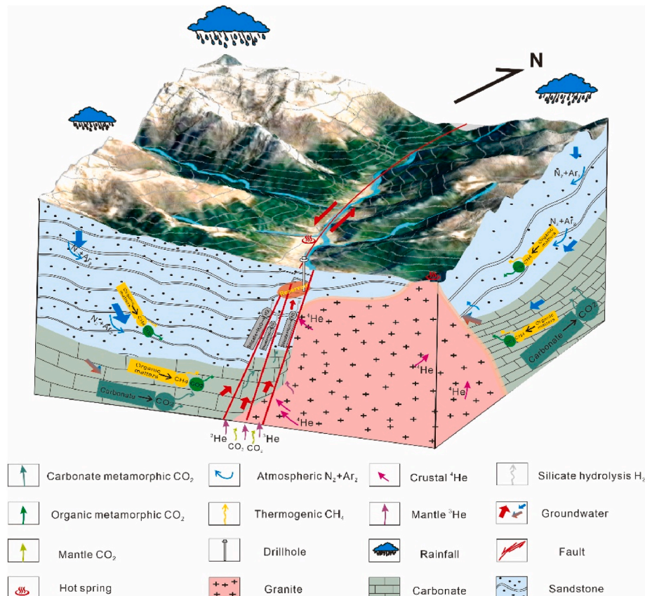
Fig. 10. Conceptual model for hydrothermal volatiles evolution in Yulingong geothermal system.
