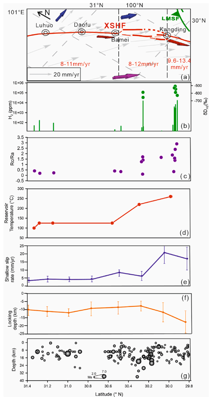
Fig. 6. (a) Summary of fault trace for each segment of the XSHF with best constrained late Quaternary slip rates in red at bottom of figure (modified from Ref. [49]). Red arrows show southeastward slip rate increase. Grey arrows show GPS vectors relative to stable Eurasia [108]. Blue and purple 3D arrows show block movement on each side of the XSHF with their appropriate length according to GPS velocities. The (b) \text{H}_2 concentrations (represented by green bars) and (c) \text{Rc/Ra} values (represented by green dots) of the samples in this study. (d) The reservoir temperatures at Luhuo, Daofu, Bamei, Zhonggu, and Yulingong estimated by Tian et al. [39]. Spatial variations in (e) shallow aseismic slip rate and (f) locking depth inverted from Interferometric Synthetic Aperture Radar (InSAR) data [106]. (g) The focal depths of historical earthquakes with the increasing radius of bubbles represents the increase of earthquake magnitude, detailed information listed in Table S1.
