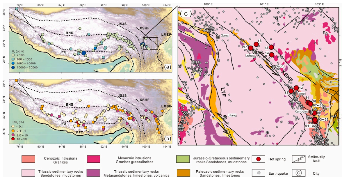
Fig. 1. (a) Summary of the \text{H}_2 and (b) \text{CH}_4 contents reported in previous studies about the Tibetan Plateau; (c) a geological sketch map of near the XSHF. Abbreviations for faults are as follows: MFT, the Main Frontal thrust; IYS, the Indus-Yarlung suture; BNS, the Bangong-Nujiang suture; JSJS, the Jinshajiang suture; LMSF, the Longmenshan Fault; LTF, the Litang Fault.
