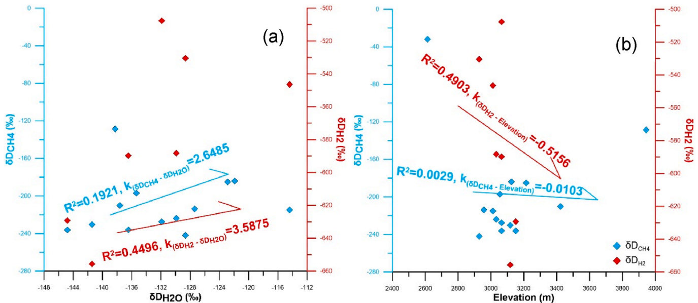
Fig. 4. Plot of \delta^2\text{D}_{\text{CH}_4} and \delta^2\text{D}_{\text{H}_2} values versus \delta^2\text{D}_{\text{H}_2\text{O}} value (a) and elevation (b). The R^2 and k values represent the coefficient and the slope of the fit lines, respectively.
