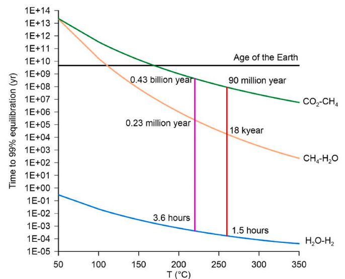
Fig. 9. The calculated time for 99 % fractional equilibration for ^{13}\text{C}/^{12}\text{C} and ^2\text{H}/^1\text{H} between \text{CO}_2 , \text{CH}_4 , \text{H}_2\text{O} and \text{H}_2 as a function of temperature in aqueous liquid. The calculations are based on rate expressions for \text{CH}_4\text{-CO}_2 (green line) [135], \text{CH}_4\text{-H}_2\text{O} (orange line) [140], and \text{H}_2\text{O-H}_2 (blue line) [133], which were compiled by Ref. [115]. The black, red and pink lines represent the age of the Earth (4.6 billion years) [141], and the reservoir temperature of 260 °C and 220 °C, respectively.
