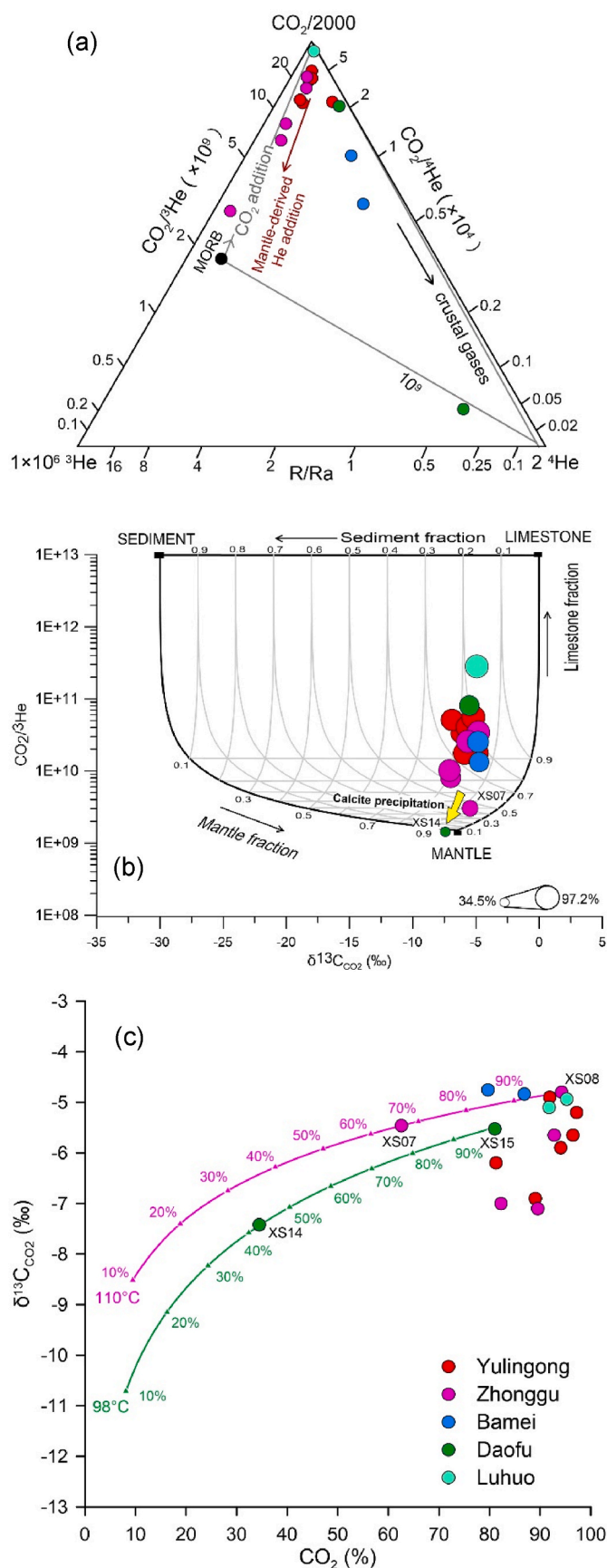
Fig. 5. (a) Triangle plot of \text{CO}_2\text{-}^3\text{He-}^4\text{He} ; (b) \text{CO}_2/{}^3\text{He-}\delta^{13}\text{C}_{\text{CO}_2} bubble plot where the increasing radius of bubble indicates the growing \text{CO}_2 content. Solid black and grey lines represent the binary mixtures between the different end-member values. Grey dashed lines with triangles show predicted calcite fractionation model [80] trends for \text{CO}_2 loss by calcite precipitation at 100 °C (as % lost carbon), assuming a mantle starting composition of \delta^{13}\text{C} = -6.5 \text{ ‰} and \text{CO}_2/{}^3\text{He} = 2 \times 10^9 ; (c) Plot of \delta^{13}\text{C}_{\text{CO}_2} values versus \text{CO}_2 contents. The pink and green solid lines labeled 110 °C and 98 °C represent isotopic and elemental fractionation of carbon during calcite precipitation from an initial condition represented by the samples of XS08 and XS15, respectively. The triangles are labeled with the fraction of remaining \text{CO}_2 .
